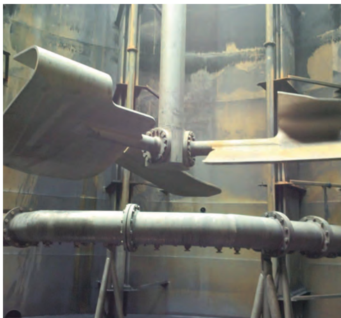
Ekato COMBIJET
